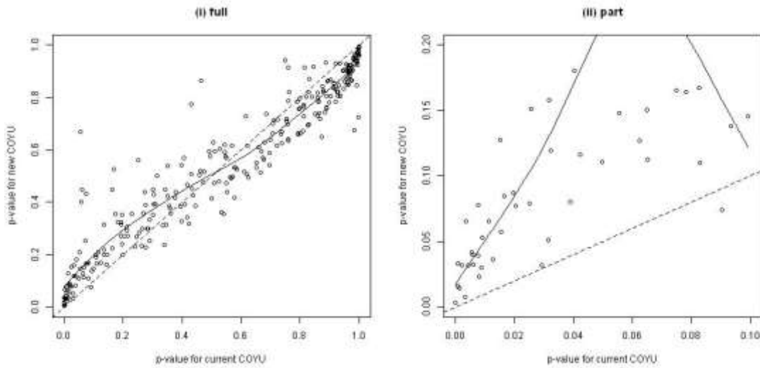
Figure A12: Comparison of p-values for UK field pea semi-leafless-type data sets; solid line is fitted curve, dashed line shows equality between the p-values
