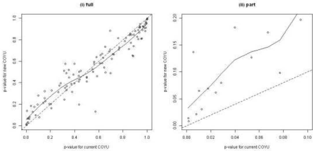
Figure A3: Comparison of p -values for France data set; solid line is fitted curve, dashed line shows equality between the p -values
