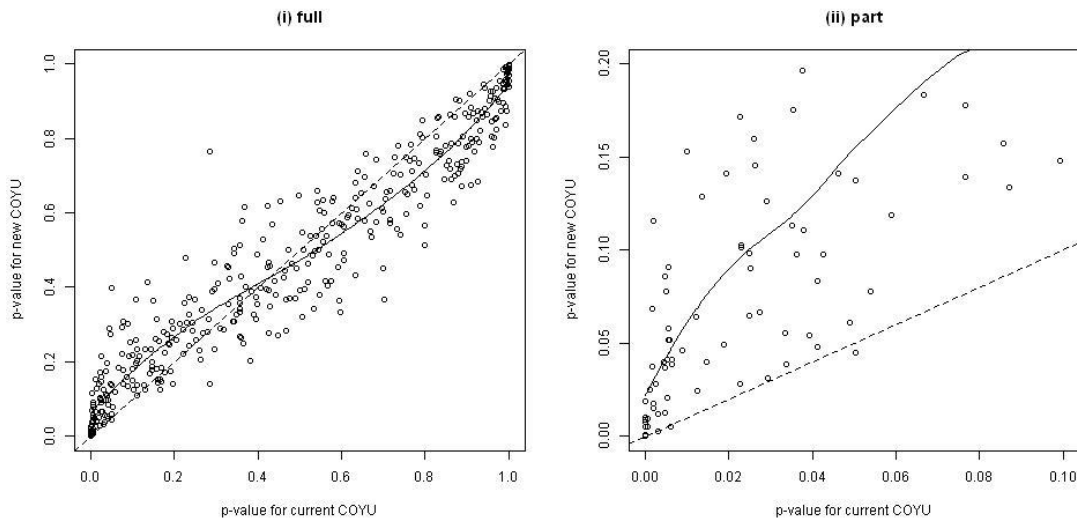
Figure A12: Comparison of p-values for the United Kingdom field pea semi-leafless-type data sets; solid line is fitted curve, dashed line shows equality between the p-values
