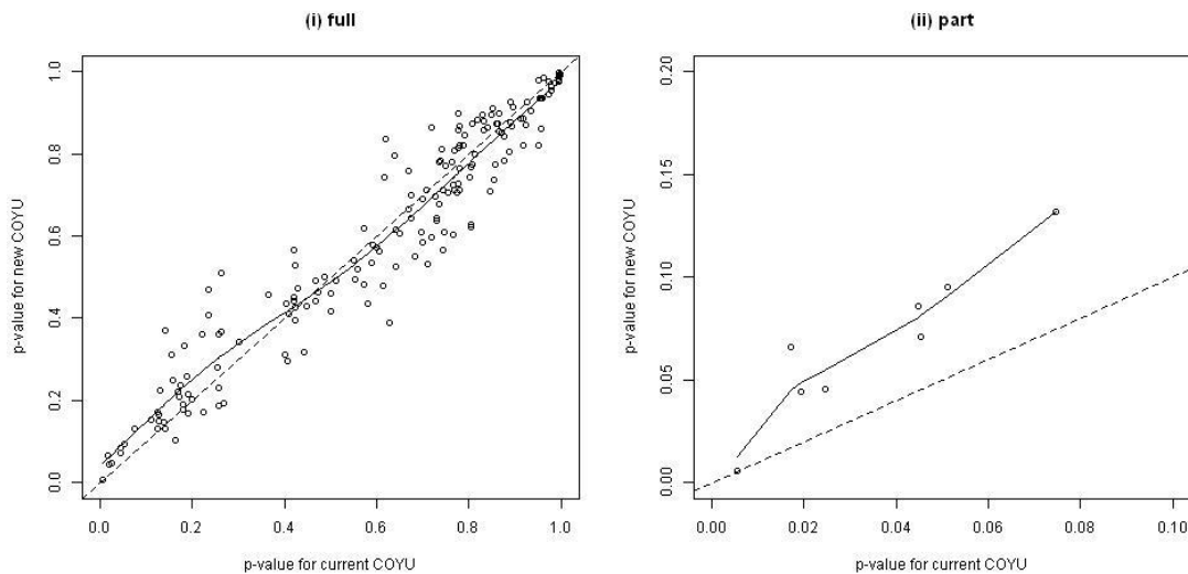
Figure A10: Comparison of p-values for the United Kingdom oilseed rape composite data set; solid line is fitted curve, dashed line shows equality between the p-values
