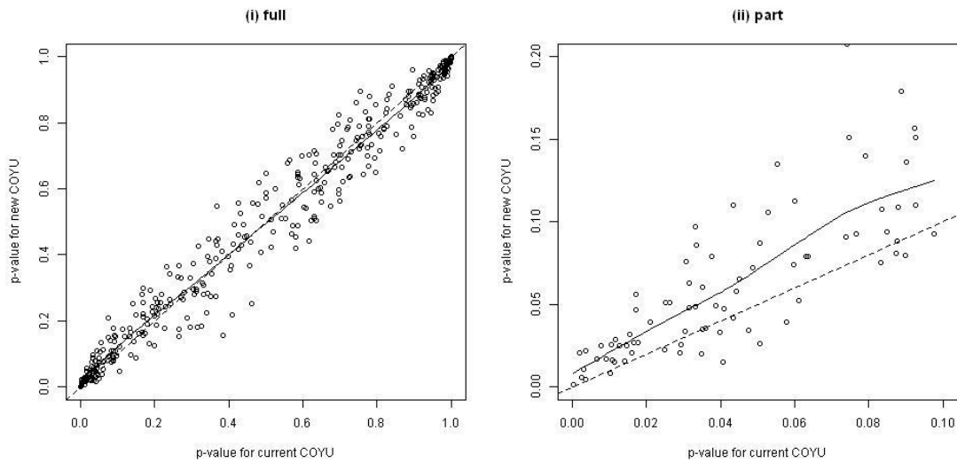
Figure A7: Comparison of p-values for the United Kingdom oilseed rape lines data set; solid line is fitted curve, dashed line shows equality between the p-values
