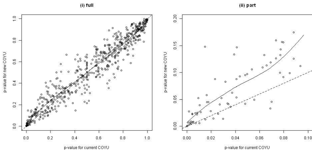
Figure A9: Comparison of p-values for the United Kingdom oilseed rape hybrids data set; solid line is fitted curve, dashed line shows equality between the p-values
