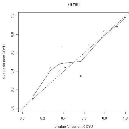
Figure A10: Comparison of p-values for the United Kingdom oilseed rape composite data set; solid line is fitted curve, dashed line shows equality between the p-values
