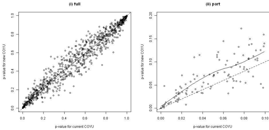
Figure A6: Comparison of p-values for the United Kingdom perennial ryegrass tetraploid data set; solid line is fitted curve, dashed line shows equality between the p-values
