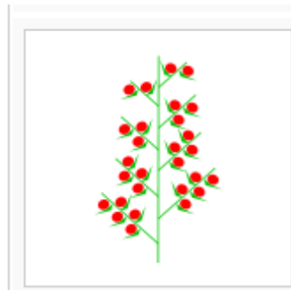
compound spike
