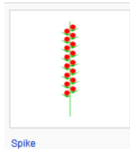
Spike
