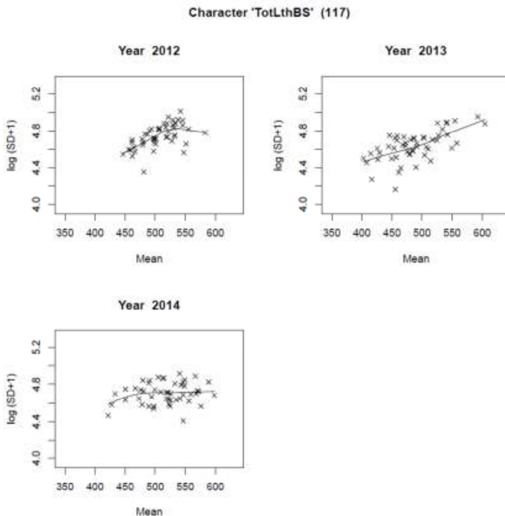
Figure A1: Spline fits of uniformity to level of expression for characteristic 117 Perennial Ryegrass Tetraploid Intermediates – data from UK
