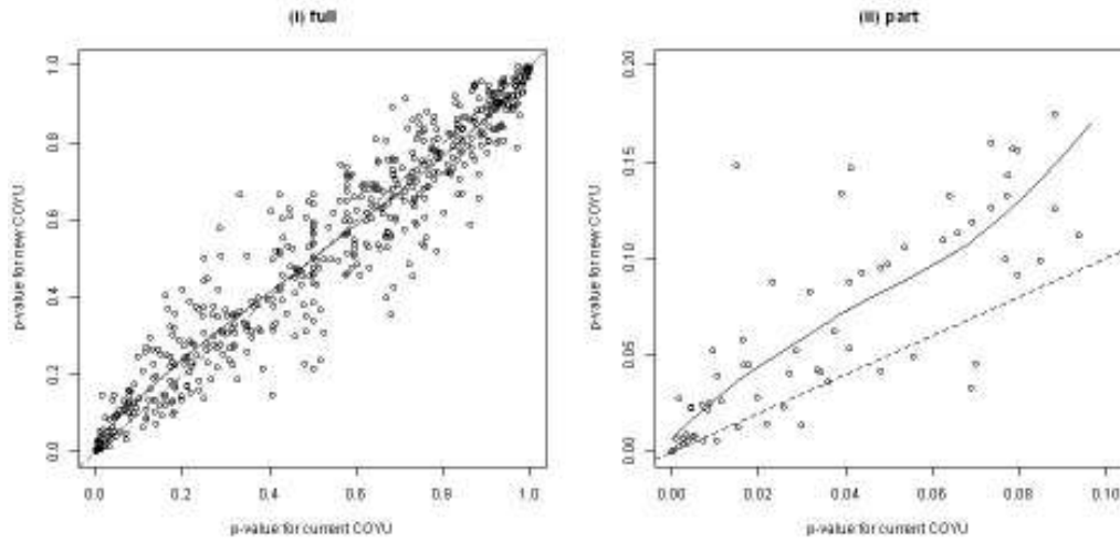
Figure A9: Comparison of p -values for UK oilseed rape hybrids data set; solid line is fitted curve, dashed line shows equality between the p -values
