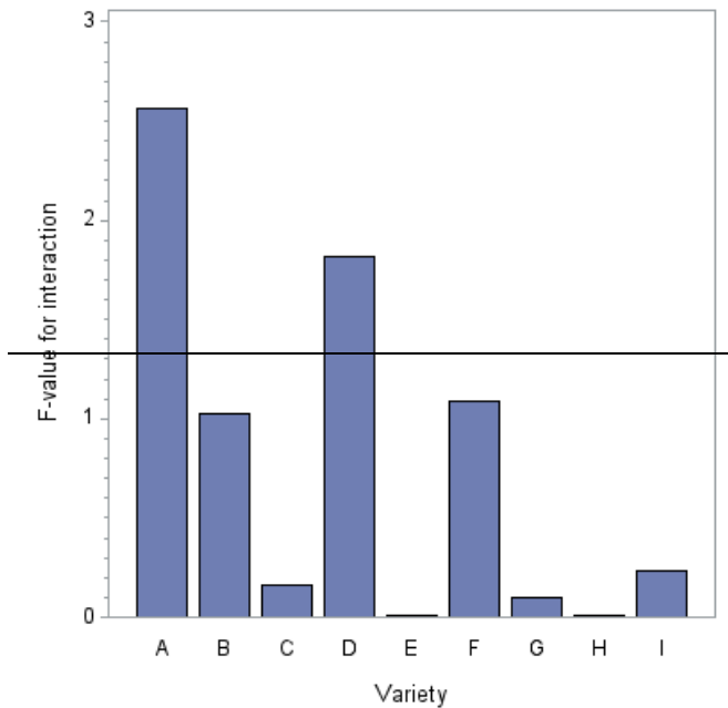
Figure 2 F_4 -values for each variety's contribution to the interaction for ordinal characteristic root tip of carrots
