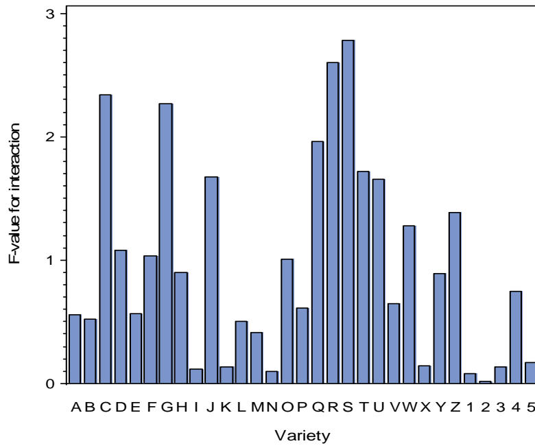
Figure 3 2 F_4 -values for each variety's contribution to the interaction for ordinal characteristic growth habit
