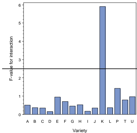
Figure 1: F_4 -values for each variety's contribution to the interaction for nominal characteristic hypocotyl color
