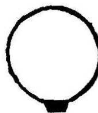
3 circular
