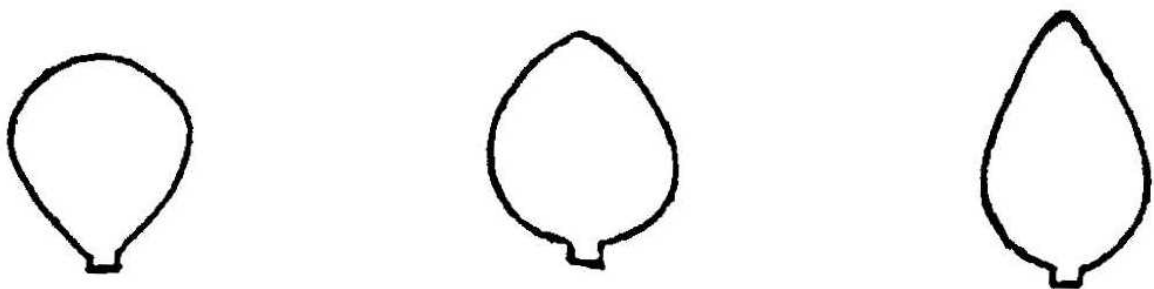
5 broad obovate
