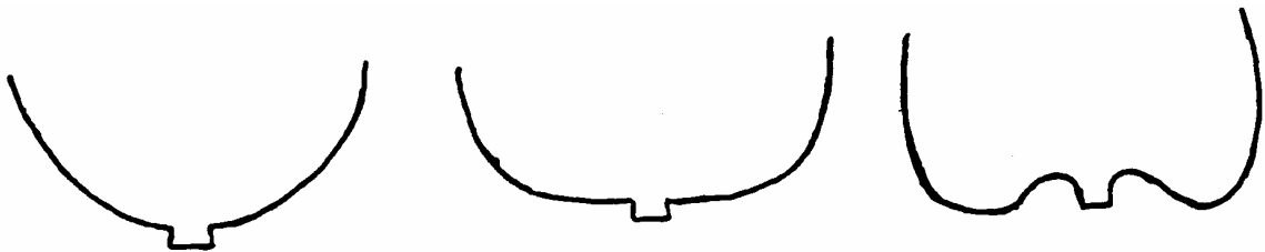
1 rounded
